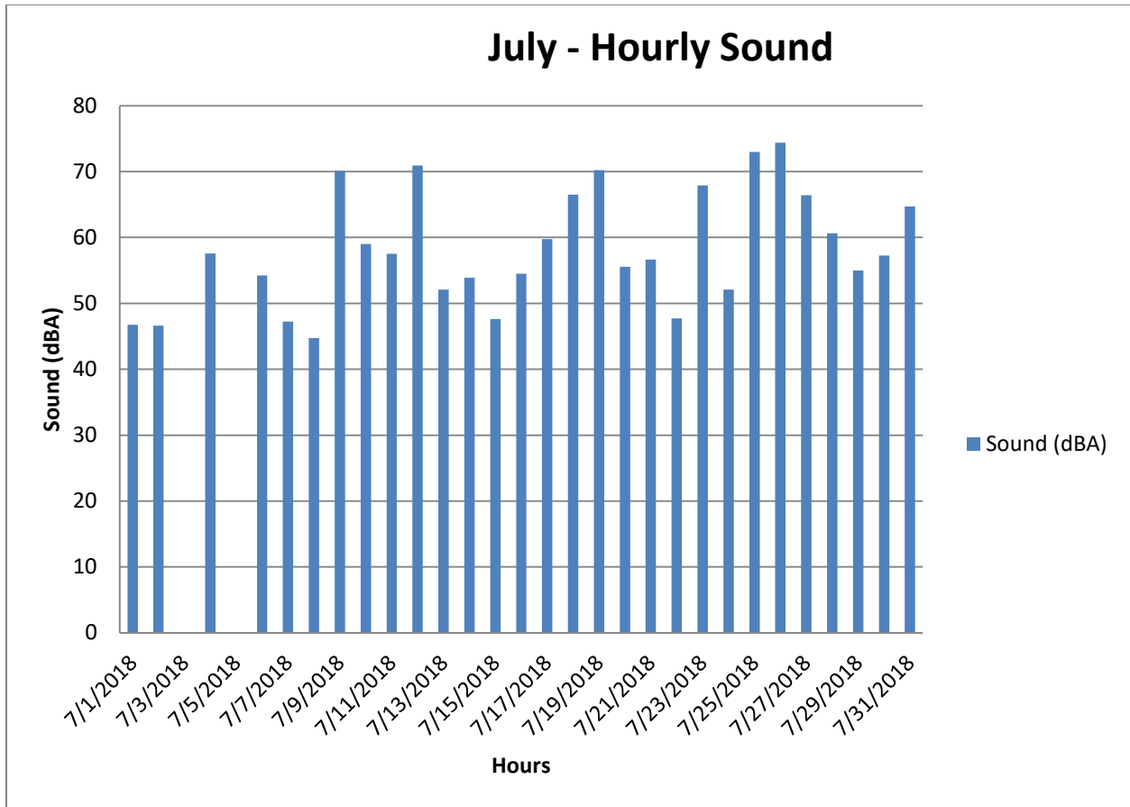
Figure D1: Hourly sound level at the STAR Pit
