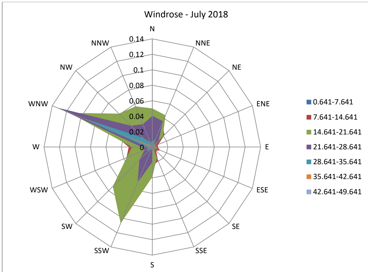
Figure B1: July 2018 wind rose from the scale house station
